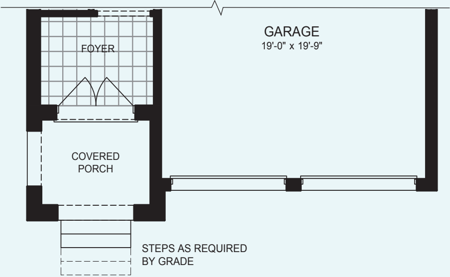
PARTIAL GROUND FLOOR PLAN ELEVATION B
