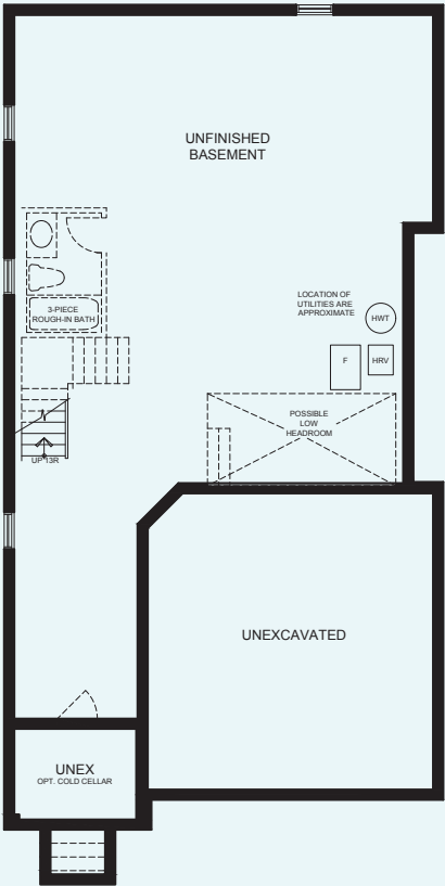
BASEMENT PLAN ELEVATION A
