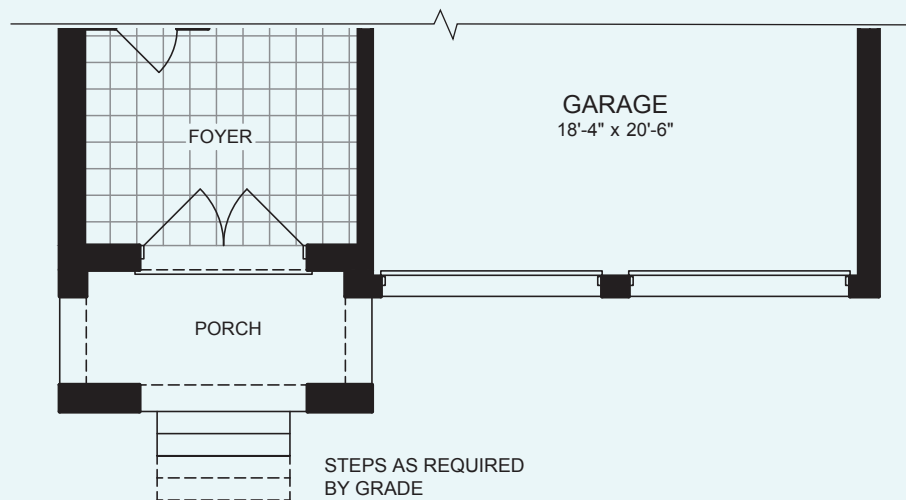
PARTIAL GROUND FLOOR PLAN ELEVATION B
