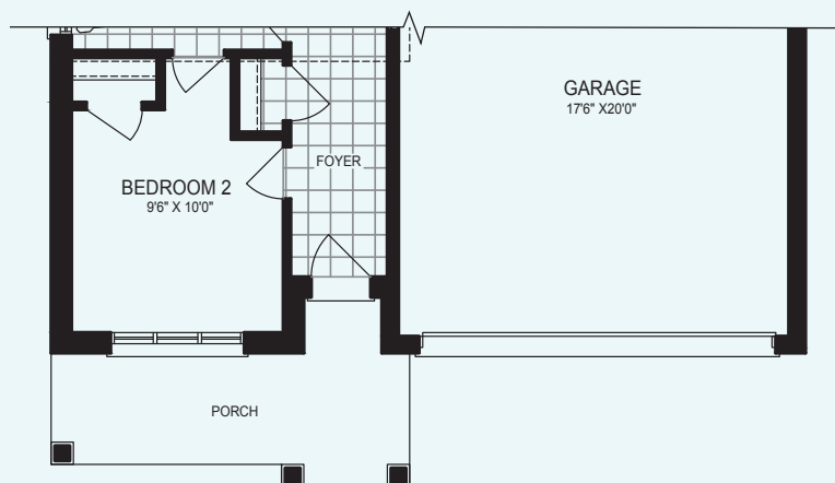
PARTIAL GROUND FLOOR PLAN ELEVATION B
