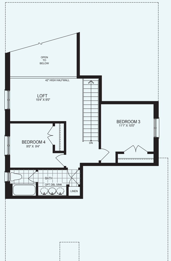
LOFT PLAN ELEVATION A
