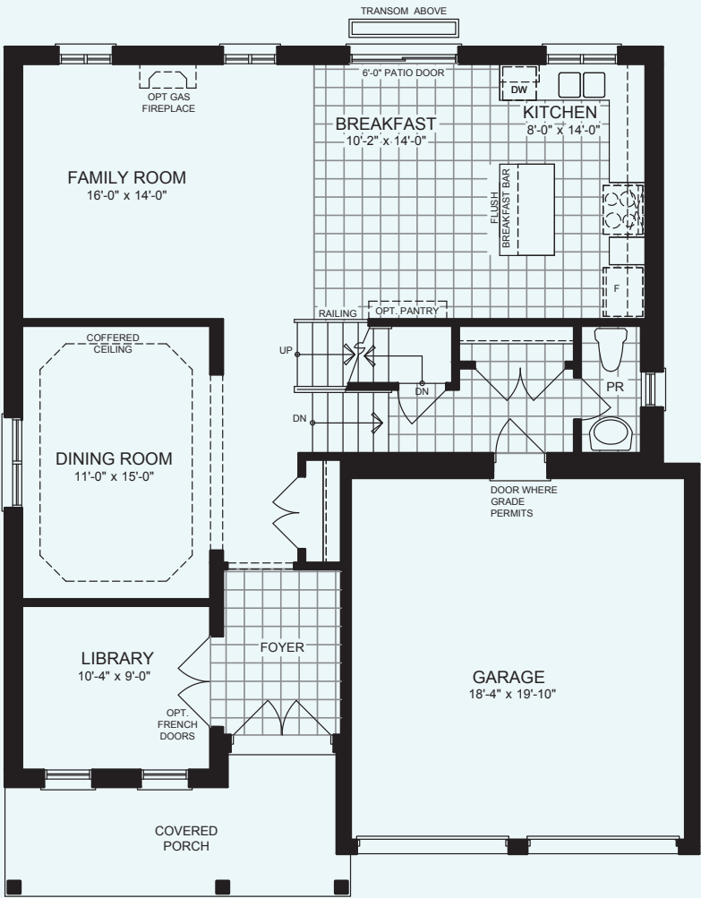
GROUND FLOOR PLAN ELEVATION A
