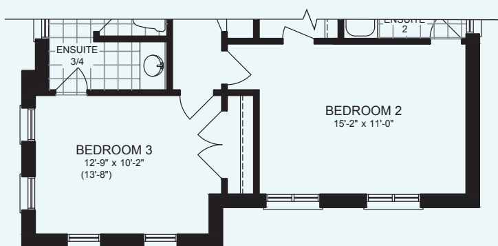
PARTIAL SECOND FLOOR PLAN ELEVATION B
