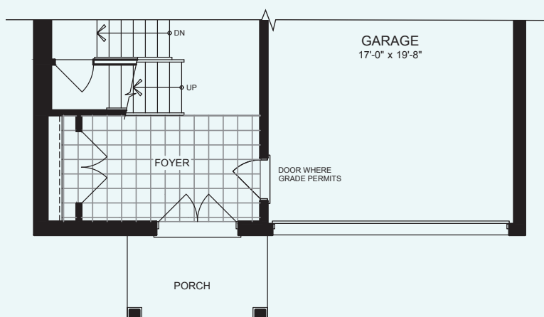
PARTIAL GROUND FLOOR PLAN LOFT B
