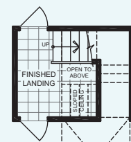
PARTIAL BASEMENT PLAN ELEVATION A & B (NO LOFT)
