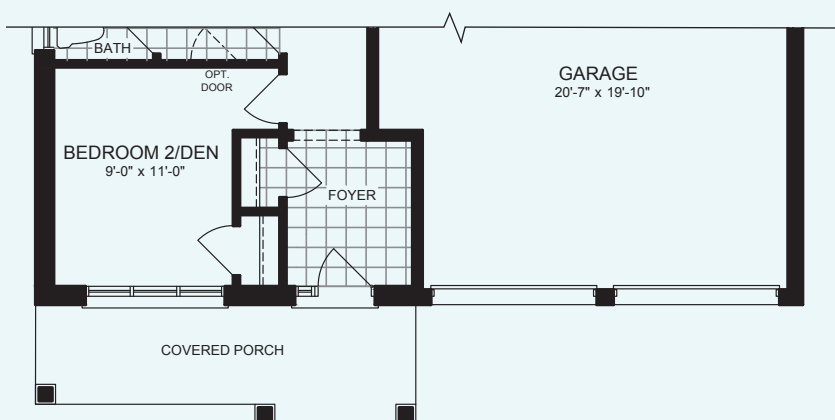
PARTIAL GROUND FLOOR PLAN LOFT B
