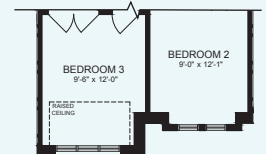
PARTIAL SECOND FLOOR PLAN ELEVATION B2
