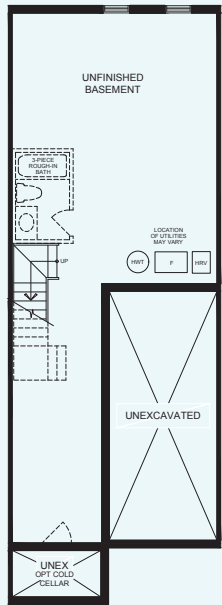
BASEMENT PLAN ELEVATION A1
