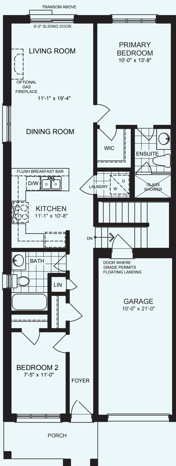
MAIN LEVEL ELEV 'A' & 'B'
