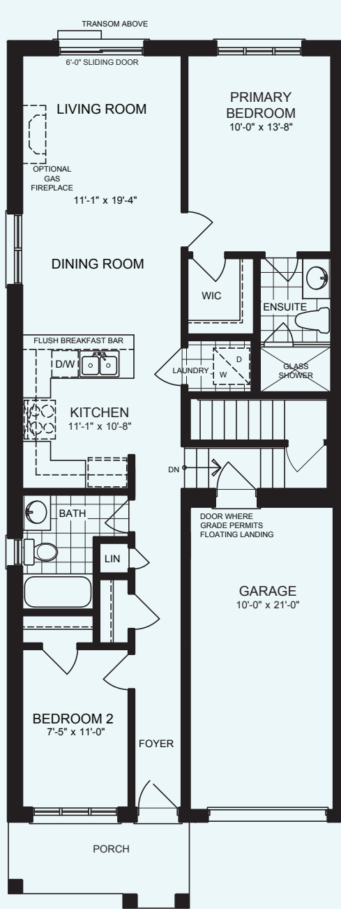
MAIN LEVEL ELEV 'A' & 'B'
