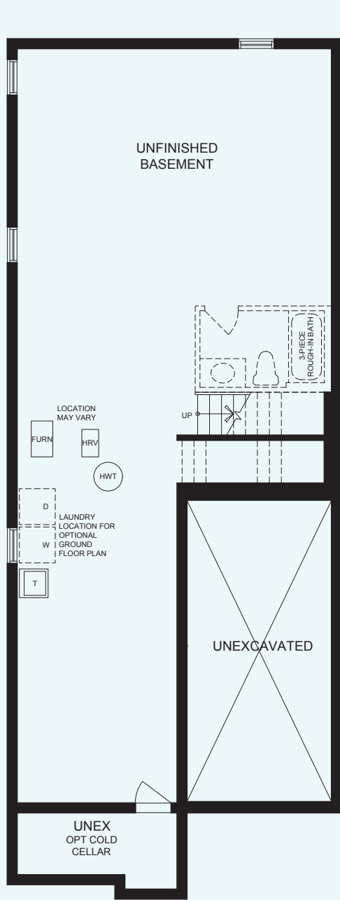
BASEMENT LEVEL ELEV 'A' & 'B'
